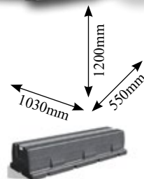
Rubber base installation block
