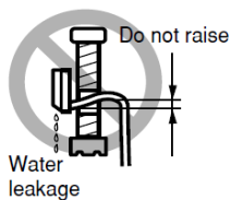
Improper installation of condensate hose
