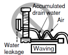
Improper installation of condensate hose
