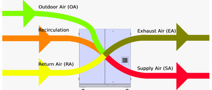
Dehumidification, air heating and filtration by Mixing
