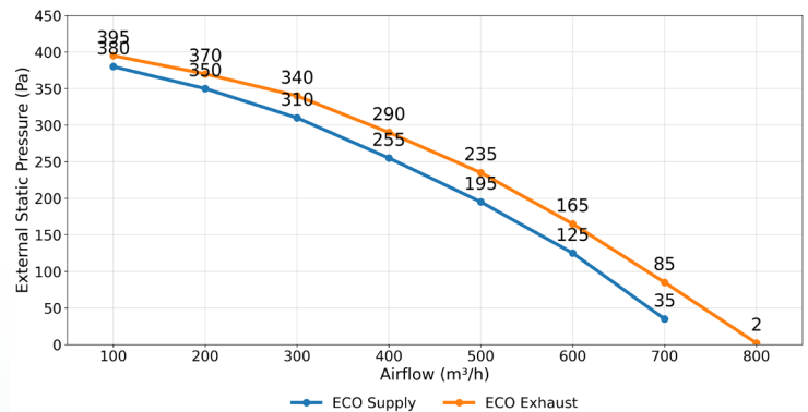
AIRFLOW AND EXTERNAL PRESSURE CHARACTERISTICS DRY X 1200 ECO
